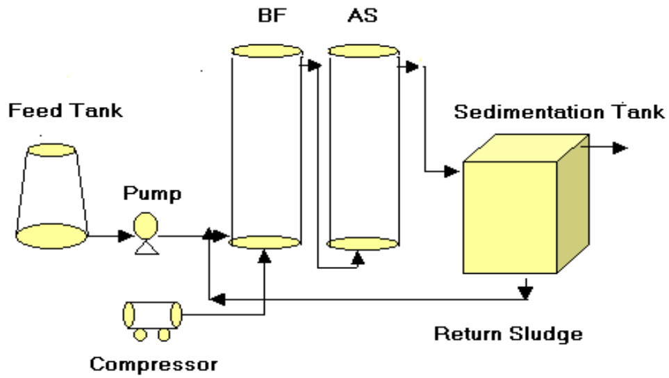
Fig. 1: Schematic and flow diagram BF/AS separated combined system
